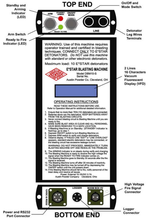
DBM 10-S Digital Blasting Machine
