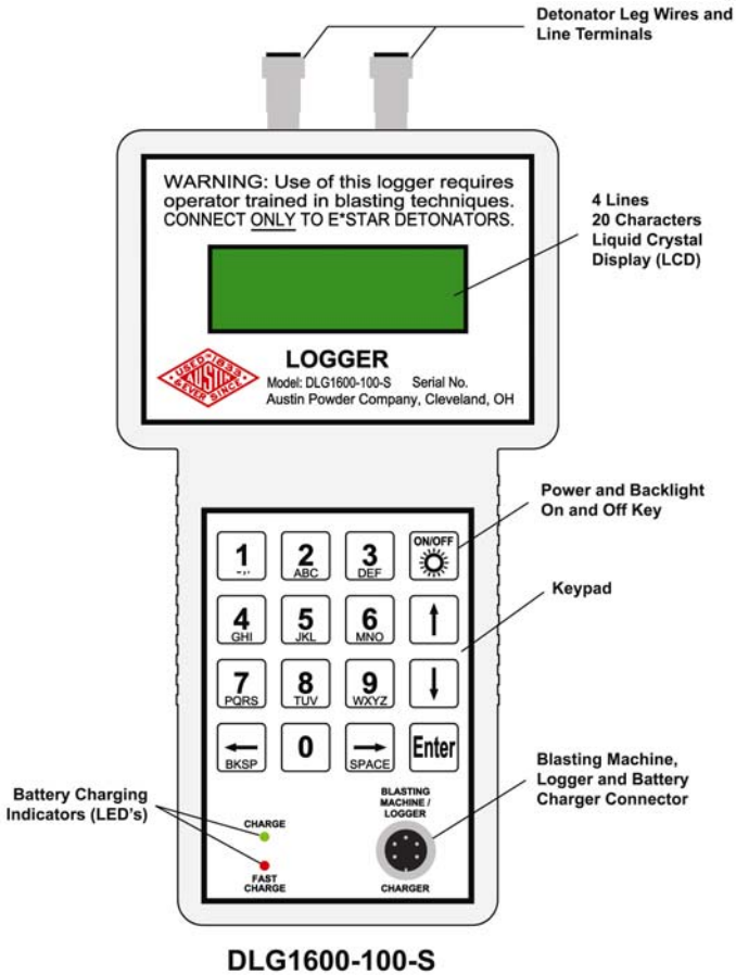
DLG1600-100S E★Star Seismic Logger
